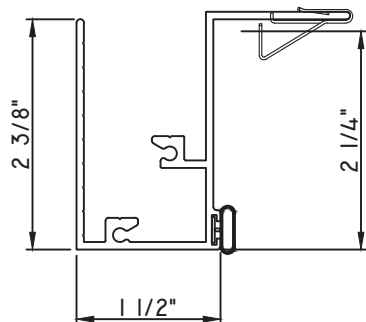
PRESET PANNING M23889 - PANNING BPN-9159 - W.S. MH8-18X1 LP - FASTENER (QTY. 8)
