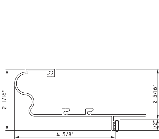
PRESET PANNING M23890 - PANNING BPN-9159 - W.S. MH8-18X1 LP - FASTENER (QTY. 8) 1974 - CLIP (6" FROM EACH CORNER & 20" O.C.)
