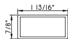
1 3/4"X7/8" M10360 SCALE 1:2
