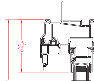
2 VERTICAL CROSS SECTION
