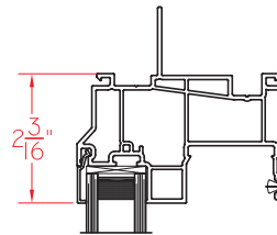
3 VERTICAL CROSS SECTION
