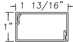
Base Clip M9762 Inside Trim M9761
