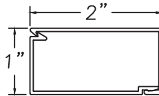
Base Clip MAX13097 Inside Trim MAX13098
