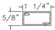
Base Clip MAX13827 Inside Trim MAX13828
