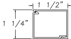
Base Clip M15266 Inside Trim M15267
