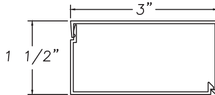
Base Clip MAX8216 Inside Trim MAX8215
