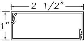
Base Clip M10121 Inside Trim MAX10120
