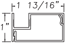
Base Clip M9762 Inside Trim M19848
