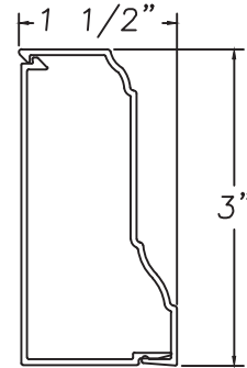
Base Clip M14253
