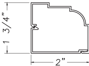
Base Clip M19884 Inside Trim M22320
