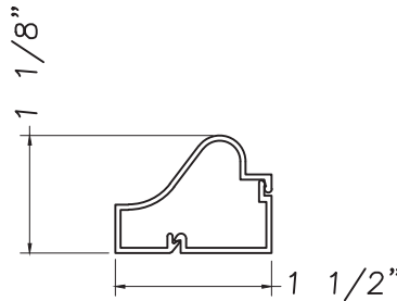
Base M22378 Trim M22438
