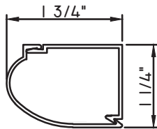
Base Clip M15266 Trim M23492
