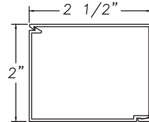
Base Clip M23403 Inside Trim M23402
