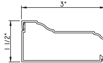
1 1/4"X1 1/2" SNAP TRIM MAX8216 - BASE CLIP M14253 - TRIM
