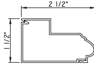
2 1/2"X1 1/2" SNAP TRIM M1984 - BASE CLIP M2212 - TRIM
