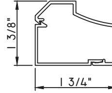
1 3/8"X1 3/4" SNAP TRIM M2078 - BASE CLIP M18301 - TRIM
