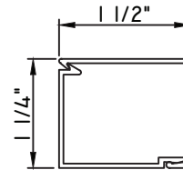
1 1/4"X1 1/2" SNAP TRIM M15266 - BASE CLIP M15267 - TRIM
