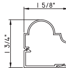
1 3/4"X1 5/8" SNAP TRIM M2144 - BASE CLIP M20526 - TRIM
