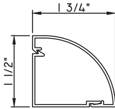
1 1/2"X1 3/4" SNAP TRIM M15266 - BASE CLIP M23501 - TRIM
