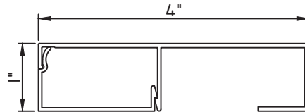
4"X1" SNAP TRIM M9762 - BASE CLIP M25176 - TRIM
