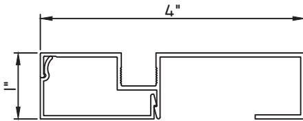
4"X1" SNAP TRIM M9762 - BASE CLIP M25175 - TRIM
