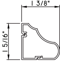
1 3/8"X1 5/16" SNAP TRIM M22378 - BASE CLIP M23568 - TRIM
