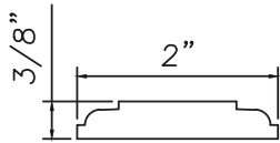
2" Raised Applied (Wood) 5142
